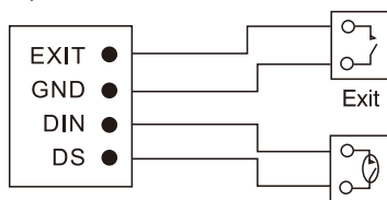
Exit/Door-detector Door-detector Sense Switch
