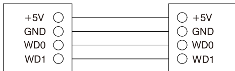
Card Reader Interface IC/ID Card Reader or Management Device
